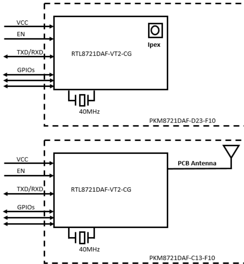
Figure 1. Block Diagram
