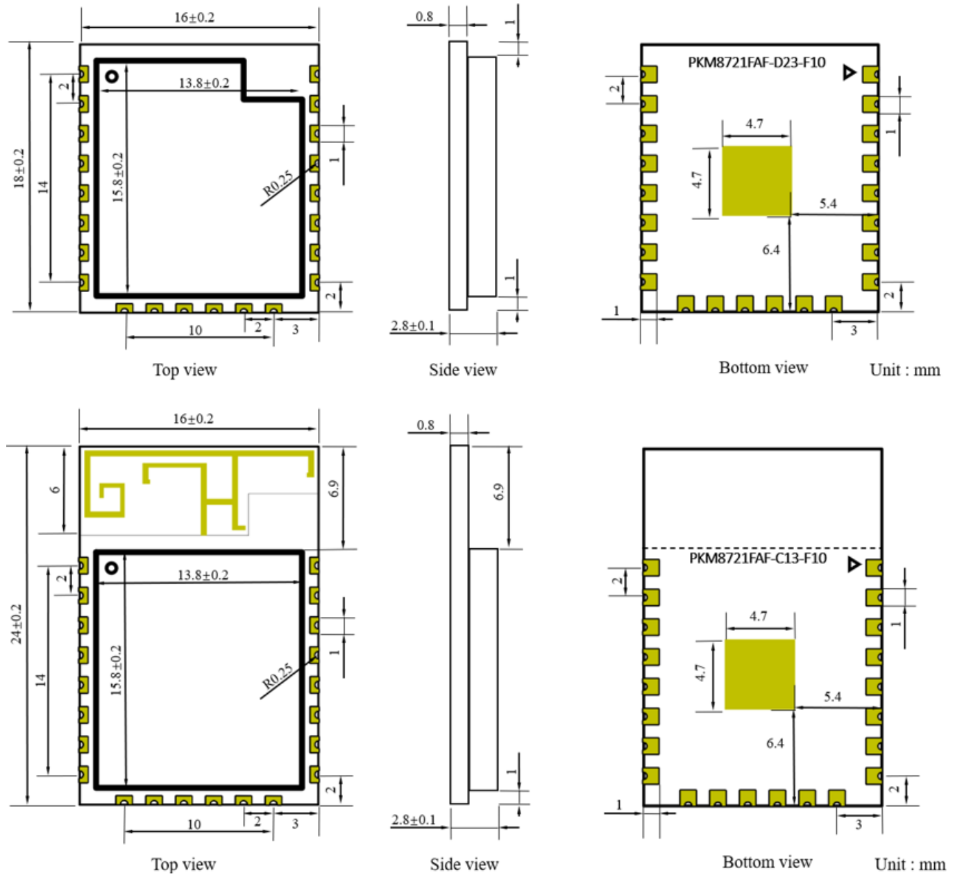
Figure 5. Module Physical Dimensions
