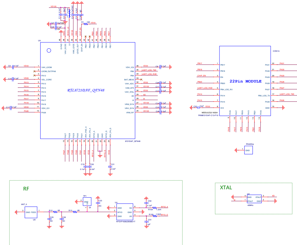
Figure 4. PKM8721DAF-C13-F10 Module Internal Schematics
