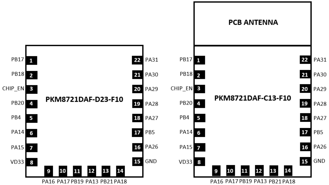
Figure 2. Module Pin Layout (Top View)
